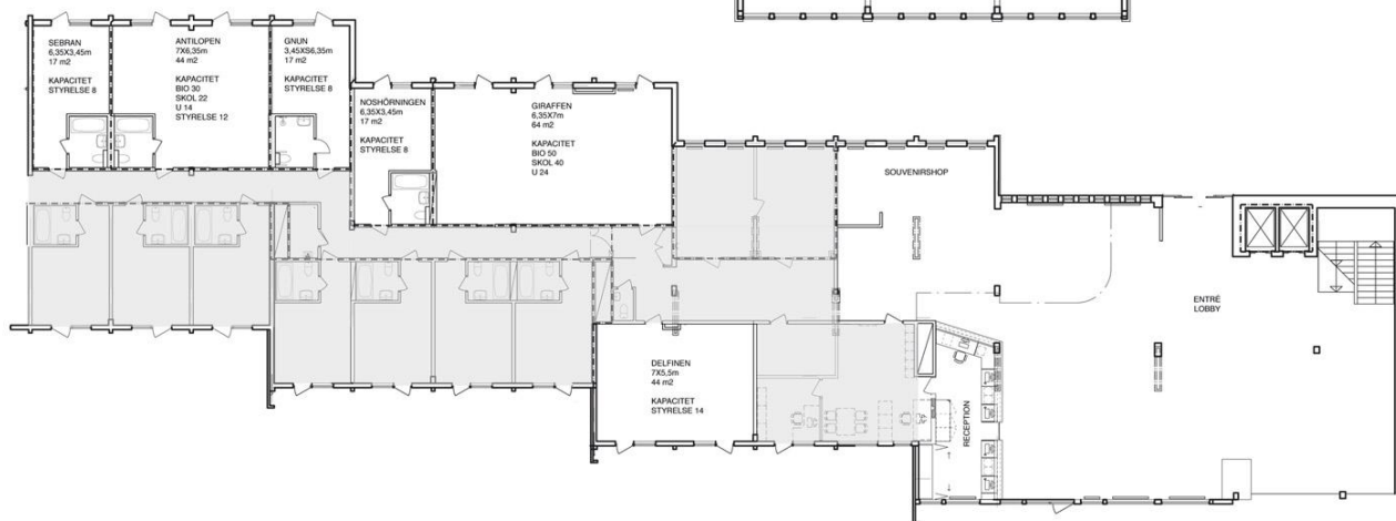
PLAN 3
